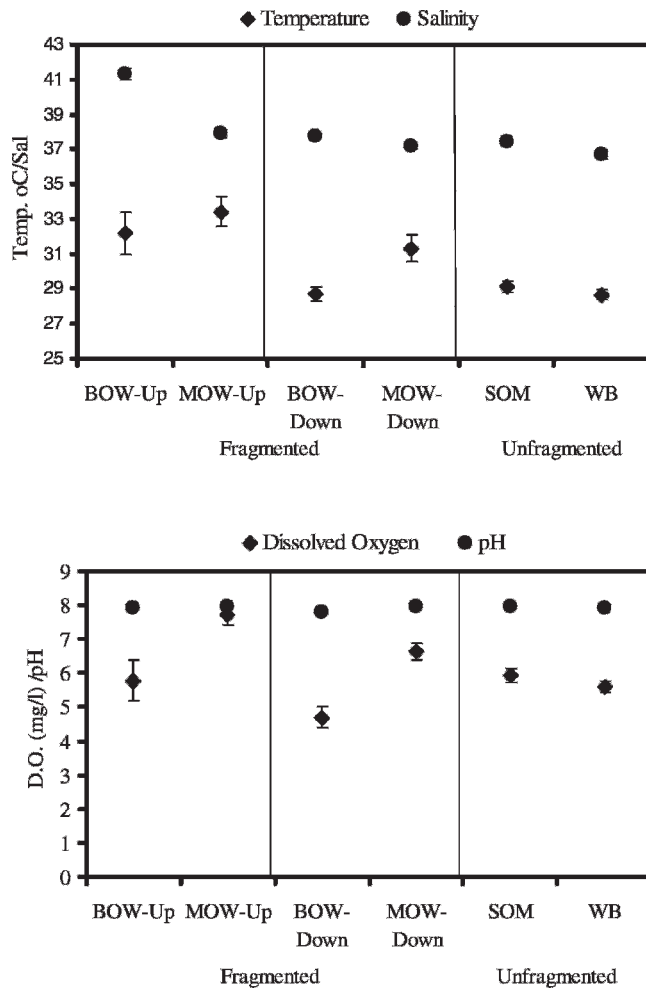
Figure 4. Means and standard deviations for A) temperature ( ^{\circ}\text{C} ), B) salinity, C) dissolved oxygen (mg/L), and D) pH. Mean values are reported for upstream (Up) and downstream (Down) areas in fragmented creeks. Tidal creek abbreviations: MOW = Man-o-War; BOW = Bowen, SOM = Somerset, WB = White Bight.
