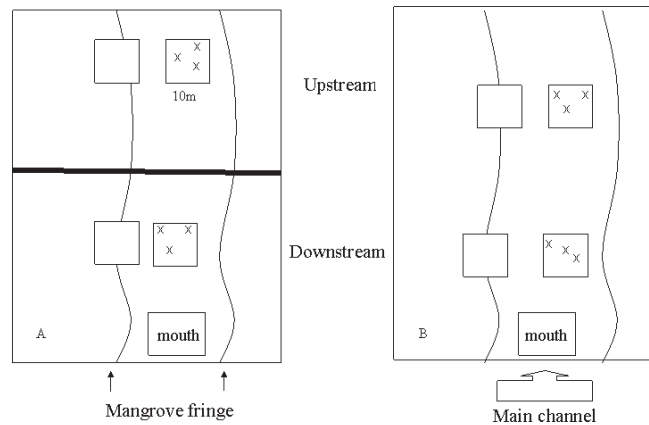
Figure 3. Schematic of transects and sampling plots upstream and downstream sites for A) fragmented and B) unfragmented tidal creeks. Plants, macroinvertebrates, and fish were surveyed in channel plots, while only fish were surveyed in mouth and side mangrove plots. Plots were 100\text{ m}^2 . Repeated plant quadrats, represented by “x”, within each plot were 1\text{ m}^2 , while repeated macroinvertebrate quadrats within each plot were 0.0625\text{ m}^2 .
