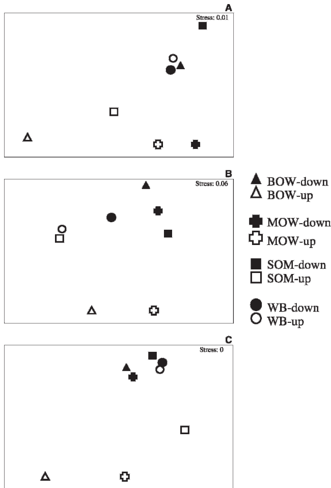
Figure 5. Non-metric Multi Dimensional Scaling results of A) Macrophytes and macroalgae, B) Macroinvertebrates, and C) Fish, presence/absence surveys in fragmented (Man-o-War and Bowen) and unfragmented (Somerset and White Bight) tidal creeks. Tidal creek abbreviations: MOW = Man-o-War; BOW = Bowen, SOM = Somerset, WB = White Bight. All quadrat data were analyzed as presence/absence in upstream and downstream locations in each tidal creek.
