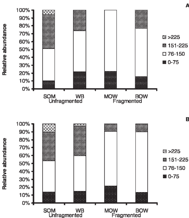
Figure 6. Relative abundance of A) schoolmaster snapper ( Lutjanus apodus ) and B) gray snapper ( L. griseus ) from four tidal creeks. Tidal creek abbreviations: MOW = Man-o-War; BOW = Bowen, SOM = Somerset, WB = White Bight. Data were obtained by determining the mean densities of each size class from all survey plots in each creek (Table 1). Significance values for MANOVA comparisons among creeks are found in Table 2.
