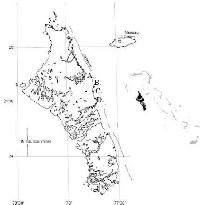
Figure 1. Line drawing of Andros Island, Bahamas. Surveyed creeks are A) Somerset, B) Bowen, C) Man-o-War, and D) White Bight.
